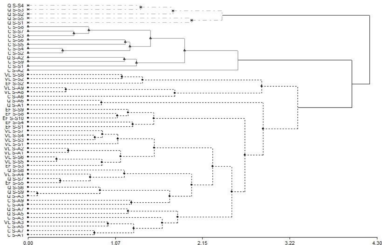
Figure 1. Dendrogram of classification of the types of honey studied according to the content of trace elements by region and season. Euclidean distance and ward aggregation method were used. C: Los Cerrillos; Q: Quebrada de los Cuervos; EF: Esteros de Farrapos; VL: Valle del Lunarejo; S-S: spring-summer; S-A: summer-autumn
