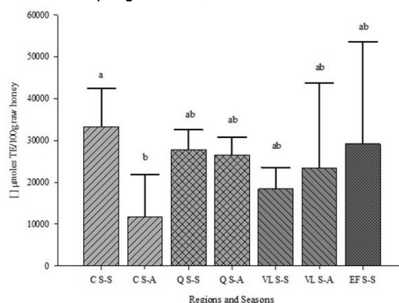
Figure 4. Antioxidant capacity ( \mu moles TE/100g honey) by region and season. The values represent the mean \pm SEM (n=7-10). Different letters indicate significant differences between regions and seasons ( p < 0.05 ). C: Los Cerrillos; Q: Quebrada de los Cuervos; EF: Esteros de Farrapos; VL: Valle del Lunarejo; S-S: spring-summer; S-A: summer-autumn
