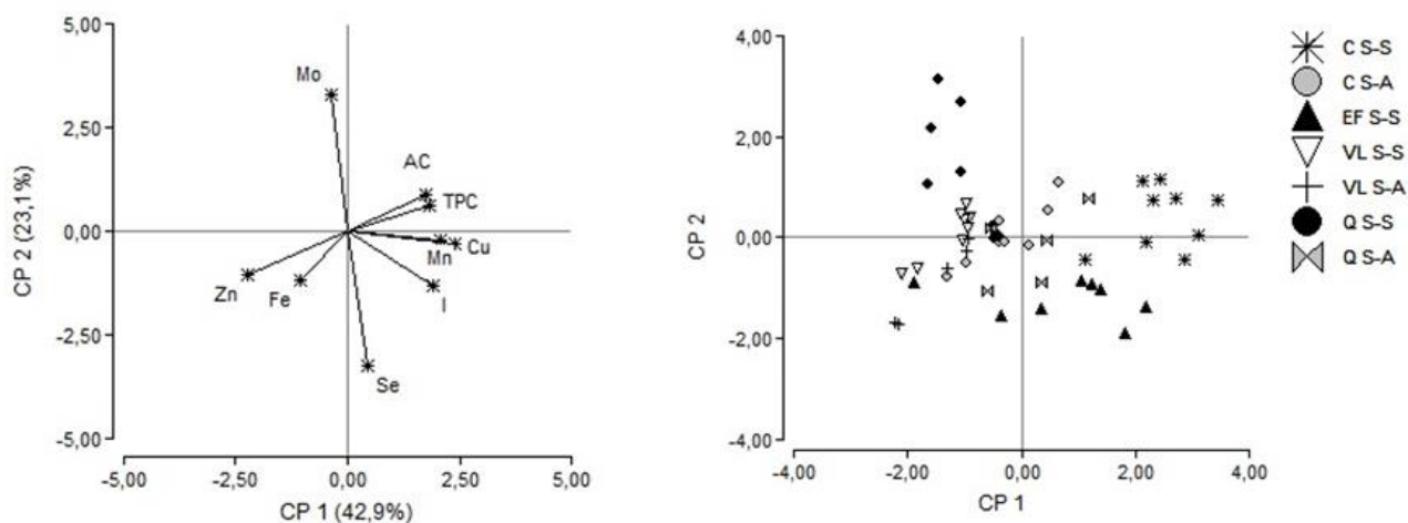
Figure 2. Analysis of main components (PCA) of the types of honey studied according to the content of trace elements, total polyphenols and antioxidant capacity by region and season. (Left: PCA distribution of variables; right: PCA distribution of honey samples). C: Los Cerrillos; Q: Quebrada de los Cuervos; EF: Esteros de Farrapos; VL: Valle del Lunarejo; S-S: spring-summer; S-A: summer-autumn
