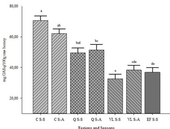
Figure 3. Total polyphenol content (TPC; mg GAEq/100g) by region and season. The values represent the mean \pm SEM (n=7-10). Different letters indicate significant differences between regions and seasons ( p < 0.05 ). C: Los Cerrillos; Q: Quebrada de los Cuervos; EF: Esteros de Farrapos; VL: Valle del Lunarejo; S-S: spring-summer; S-A: summer-autumn
